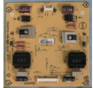
LED driver PWB (1pcs)
